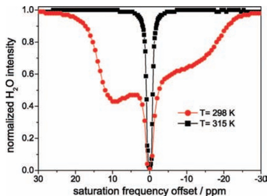
Figure 1. The Z-spectra ( B_1 = 4.5 \mu\text{T} ) of liposomes containing [Tm(hpdo3a)(H 2 O)] and NH 4 PF 6 at 298 K (red dots) and 315 K (black squares) ( B_0 = 7 \text{ T} ).
