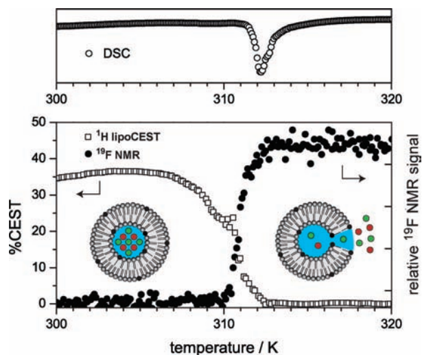
Figure 2. The ^1\text{H} CEST effect ( B_1 = 4.5 \mu\text{T} ) and the ^{19}\text{F} NMR signal intensity of liposomes containing [\text{Tm}(\text{hpdo}3\text{a})(\text{H}_2\text{O})] and \text{NH}_4\text{PF}_6 as a function of temperature at B_0 = 7 \text{ T} (lower panel). The DSC thermogram shows the melting temperature of the lipid membrane (upper panel).
